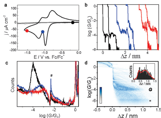
Figure 2. a) Cyclic voltammograms of NDI-BT immobilized on the Au(111) (black curve) and bare Au(111) (gray curve) in HMImpF 6 . The scan rate was 50 \text{ mV s}^{-1} . b) Typical conductance-distance traces of NDI-N (black), NDI-R (blue), and NDI-D (red). c) Conductance histogram sampled at different potential, # represents an artifact from the linear amplifier. d) Two-dimensional conductance-distance histogram of NDI-N, * represents the noise during the electrochemical STM BJ measurement. Inset: characteristic displacement histograms of NDI-N determined from the conductance region between 10^{-4.5} G_0 and 0.7 G_0 .
